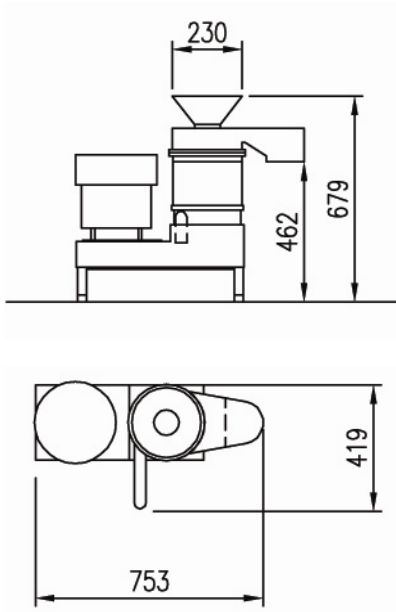
SANOVO SEC 560 Centrifuge
