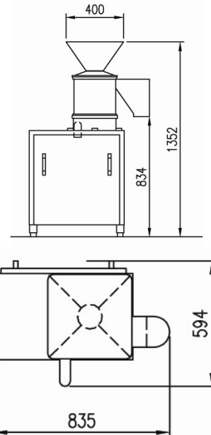
SANOVO SEC 1400 Centrifuge
