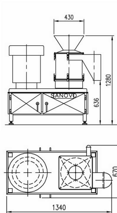
SANOVO SEC 560 Centrifuge
